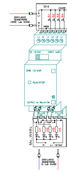
LOGO! DM8 12/24R
